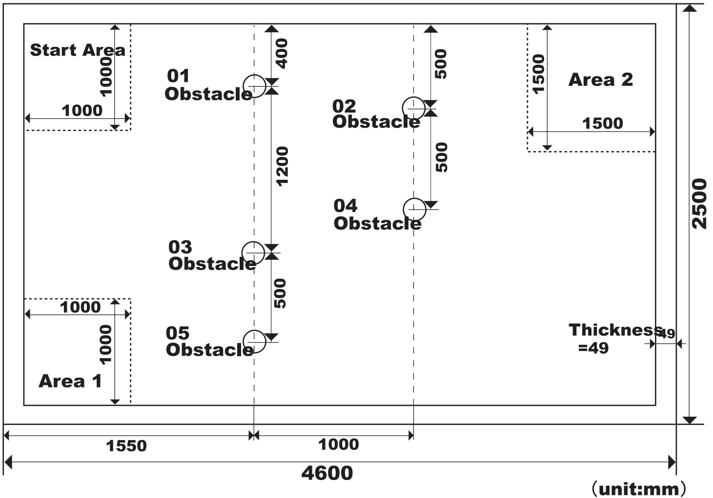
Fig.1 Contest stage plan
